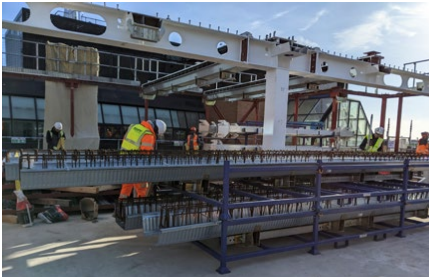
Stillage containing multiple beam shutters with reinforcement cages pre-installed at The Forge.
