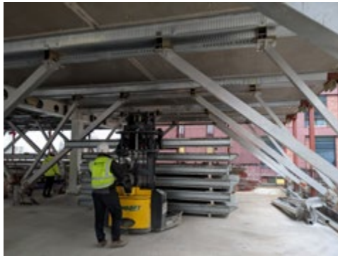
2. Shutters in place working at height.
