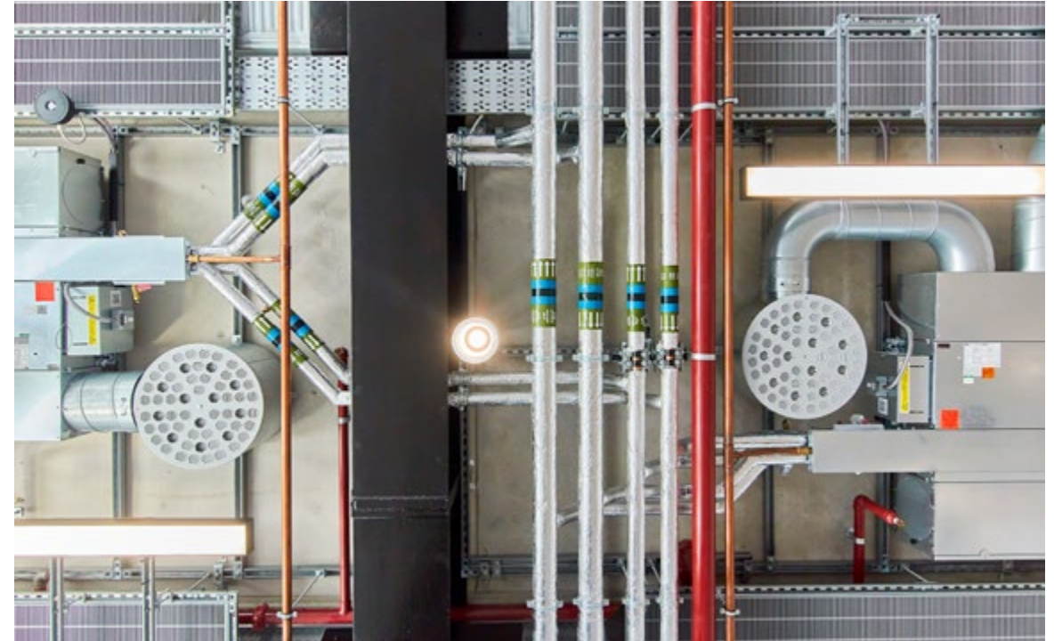
MEP attached to fixing points cast into the soffit.
