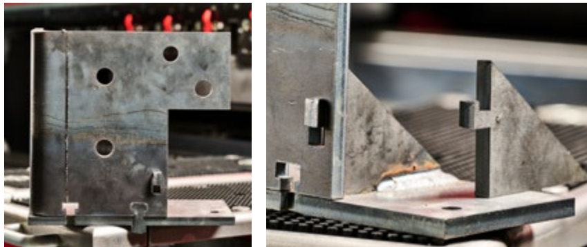
Laser cut Platform II brackets developed by the MTC
