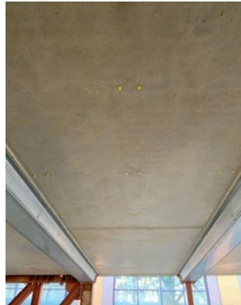
Completed soffit on-site. Note fixing points for MEP cast into slab
