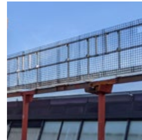
Handrails pre-attached to microcolumns
