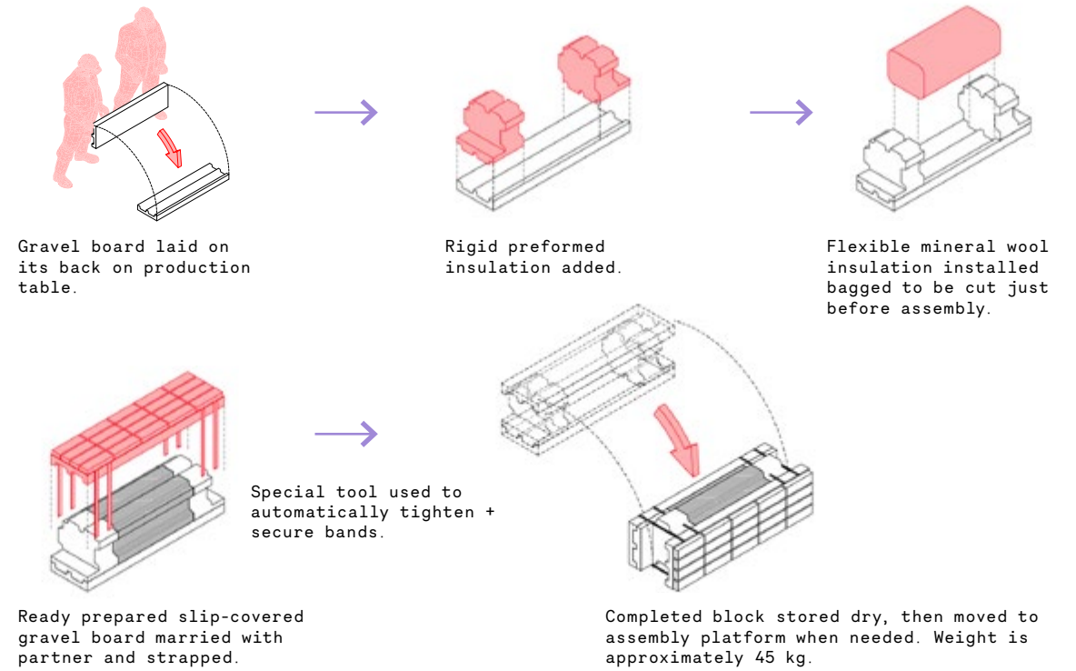
Superblock manufacturing process - Labour by cost
